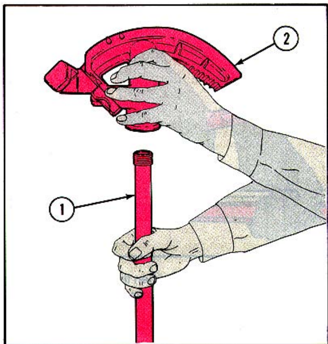
1 Install handle (1) on bender (2). A section of threaded pipe may be used as a handle.
