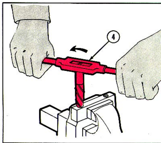
3 Remove the broken screw by turning the extractor counterclockwise. The extractor may be turned using a tap wrench or open end wrench (4).
