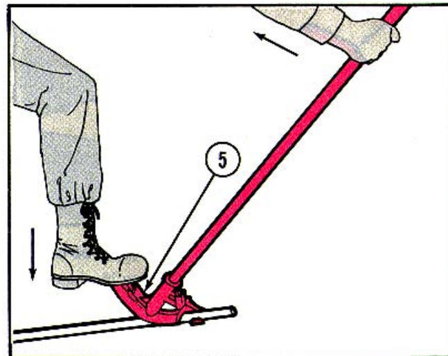
4 Place one foot on the foot rest (5) and push down with your foot while pulling back on the handle. Apply steady pressure throughout the entire bending process.
