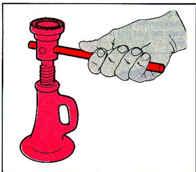
2 Turn or push the handle to the right to raise the jack, to the left to lower the jack.
