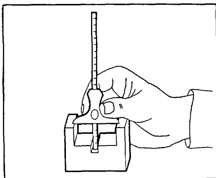
Measuring the distance from a surface to a recessed point.
