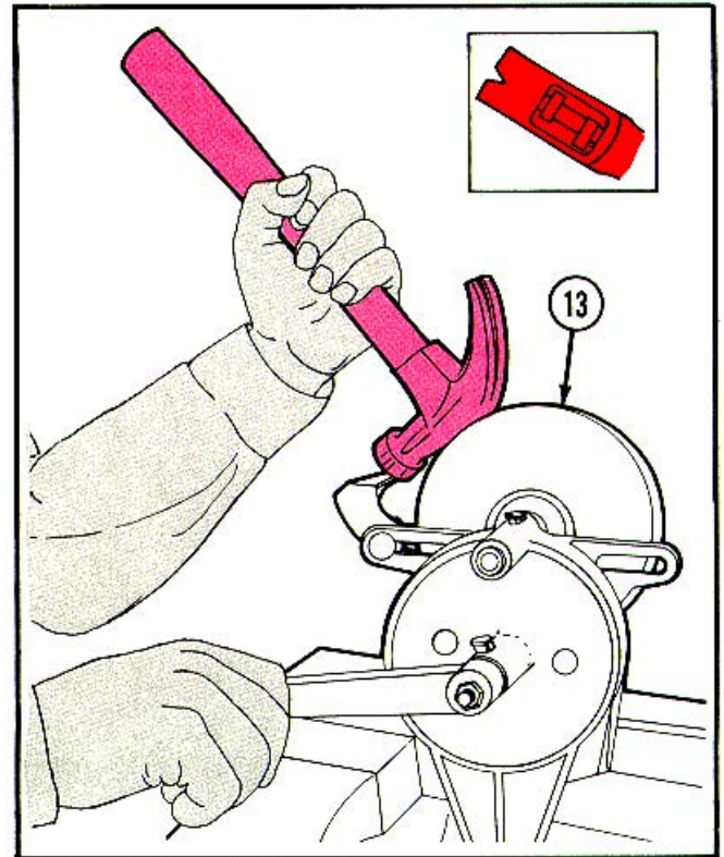
8 Remove excess portion of wedge using a bench grinder (13). Check handle. If it's tight, the task is complete. If handle is loose, repeat procedure.
