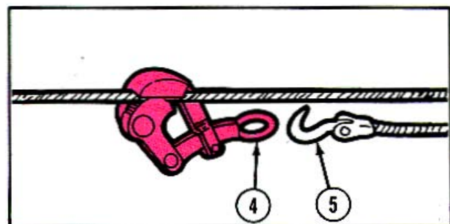
2 Fasten eye (4) to tension puller hook (5).
