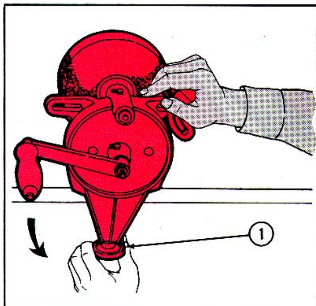
3 Position grinder where it will be used and tighten the mounting clamp (1) to hold securely on the bench.
