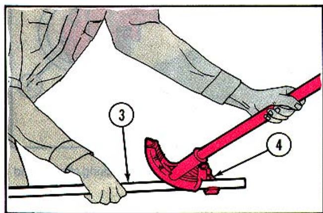
2 Tip the bender forward and slide the section of conduit (3) to be bent through the retaining hook (4).
