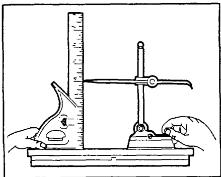
Setting gage for transfer of 4-inch vertical measurement.
