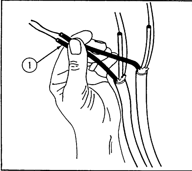
1 Using one hand, hold wires to be twisted (1) just above the point where the twist is to begin.
