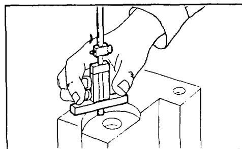
Measuring hole depth of die from a given surface.
