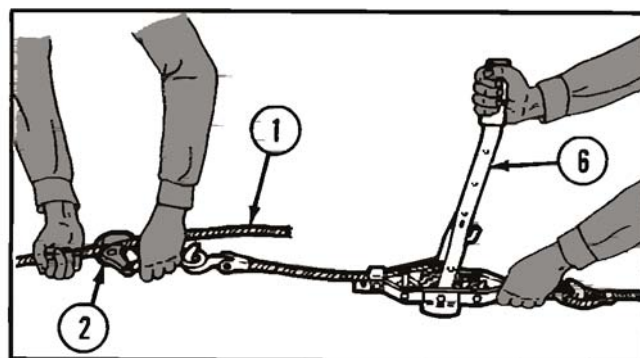
3 Hold the jaws (2) together over cable (1). Apply pressure with tension puller handle (6).
