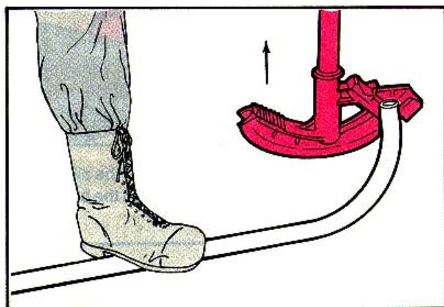
5 When desired bend has been obtained, release the pressure on the conduit by returning the handle to an upright position and slide the conduit out of the bender.
