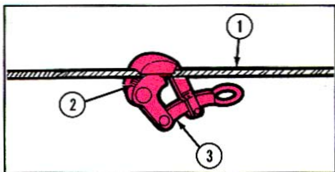
1 Place end of cable (1) between jaws (2) of cable jaw grip (3) (from jaw end of tool).
