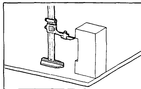
Measuring vertical distance from a plane surface.
