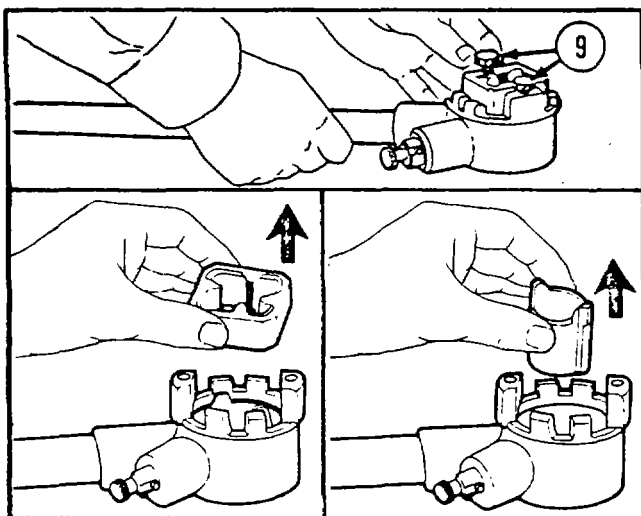
16 Disassemble the die from the ratchet handle as shown, by removing locking screws (9). Remove die and collar from ratchet head.
